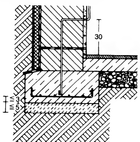
⑬ Earthing electrode in a reinforced concrete foundation
